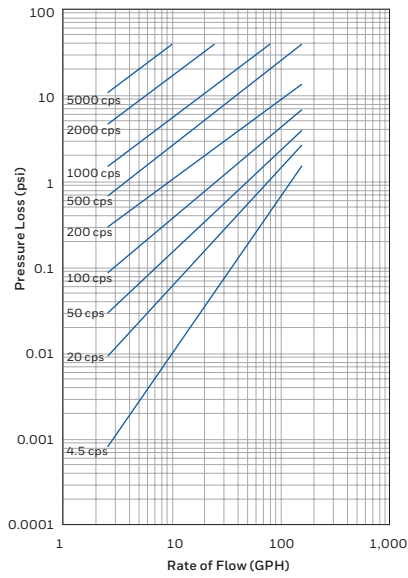
Honeywell 15 – 1/2" Oil Meter
