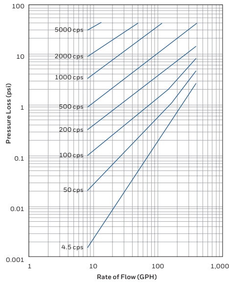
Honeywell 20 – 3/4" Oil Meter
