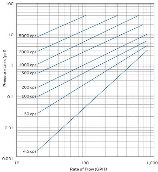
Honeywell 25 – 1" Oil Meter
