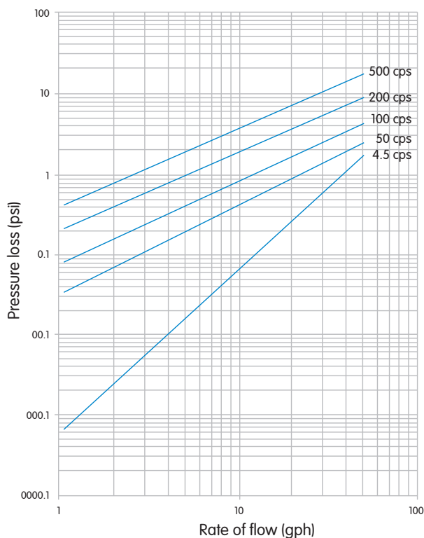
Elster 8 – 1/4" oil meter
