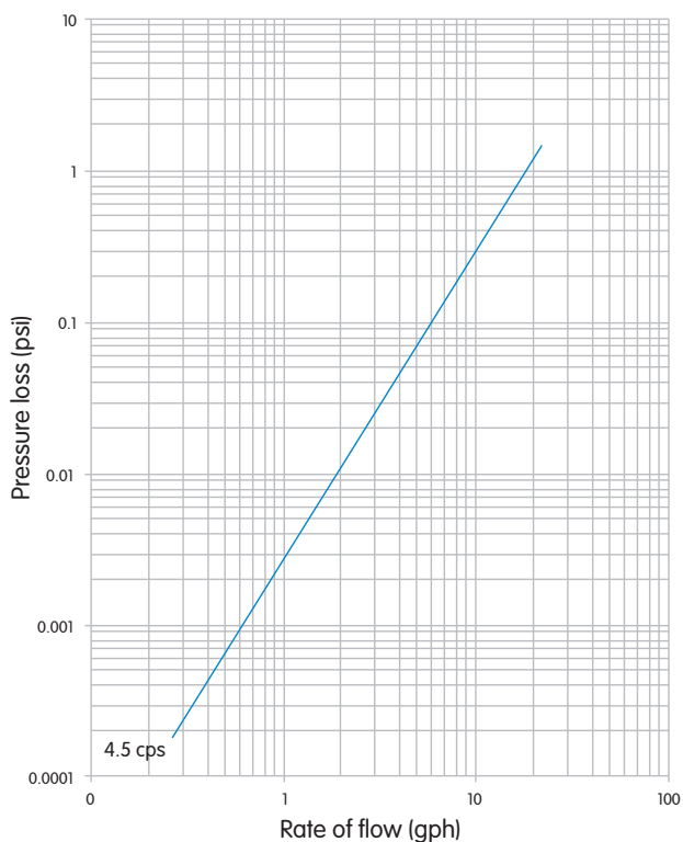
Elster 4 – 1/8" oil meter
